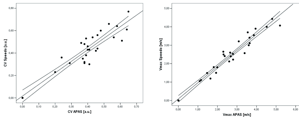
Figure 1: Linear regression models between speedo-meter system and videometric system for the velocity coefficient of variation and maximal velocity within the gait cycle.
